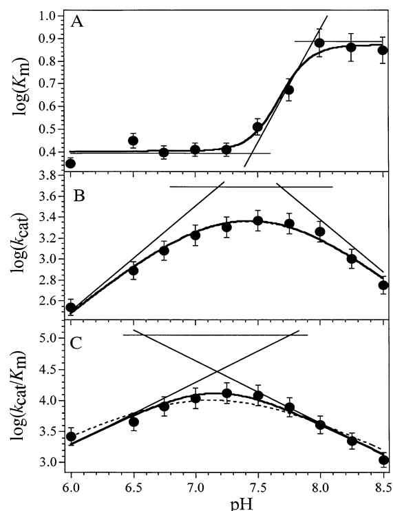
FIGURE 4: pH dependence of the kinetic parameters for the hydrolysis of MGMM by WT EcMetAP-I between pH 6.0 and 8.5. Data were fitted to eqs 4 and 5 (solid line) plots B and C, respectively. The same data were also fit to eq 10 and 11 (dashed line). (A) \log(K_m) vs. pH. The values \text{p}K_a = 7.5 \pm 0.1 and 7.9 \pm 0.1 were obtained using graphical method. The solid line represents a fit to equation describing a sigmoidal curve and was not used for calculations. (B) \log(k_{\text{cat}}) vs pH [ \text{p}K_{\text{ES1}} = 7.2 \pm 0.1 and \text{p}K_{\text{ES2}} = 7.7 \pm 0.1 , k'_{\text{cat}} = (5 \pm 1) \times 10^3 ]. (C) \log(k_{\text{cat}}/K_m) vs pH [ \text{p}K_{\text{E1}} = 7.7 \pm 0.5 and \text{p}K_{\text{E2}} = 6.6 \pm 0.5 , k_{\text{cat}}/K_m = (1.1 \pm 0.2) \times 10^5 ].
