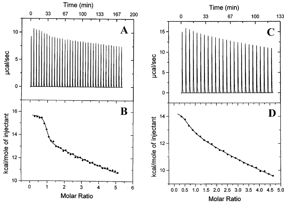
FIGURE 2: (A) ITC titration of a 70 \mu\text{M} solution of WT EcMetAP-I with a 5 mM Co(II) solution. (C) ITC titration of a 70 \mu\text{M} solution of H178A EcMetAP-I with a 5 mM Co(II) solution. (B) Fit of the ITC data for WT EcMetAP-I and (D) for H178A EcMetAP-I after subtraction of the heat of dilution. The fits were obtained using noninteracting sites model and provided an overall n value of 3, with one tight and two loose sites. Reaction conditions: 20 ^{\circ}\text{C} in 25 mM HEPES, pH 7.5, and 150 mM KCl.
