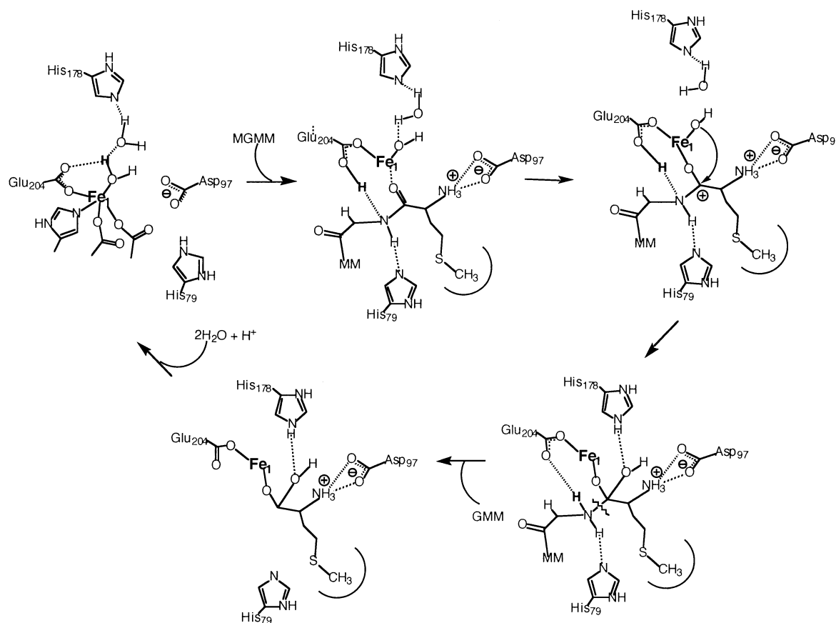
FIGURE 8: Proposed Catalytic Mechanism for EcMetAP-I .
