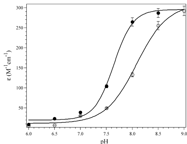
FIGURE 7: Plots of extinction coefficient ( \epsilon ) at 640 nm vs pH for wild type (○) and H178A (●) EcMetAP-I . The solid lines represent a fit to an equation of a sigmoidal curve. The midpoints of each curve provided pK_a values 8.0 and 7.6 for WT and H178A EcMetAP-I , respectively.
