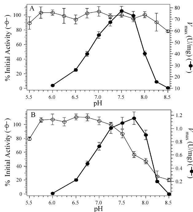
FIGURE 3: (A) Plot of V_{\max} vs pH for WT EcMetAP-I (●) and a percent of activity recovered after incubating the enzyme at the desired pH for the assay time (30 min + one minute) followed by adjustment of the pH back to 7.5 after which the specific activity was determined (○). (B) Plot of V_{\max} vs pH for H178A EcMetAP-I (●) and a percent of activity recovered after incubating the enzyme at the desired pH for the assay time (30 min + 1 h) followed by adjustment of the pH back to 7.5 after which the specific activity was determined (○). The assays were performed using 8 mM MGMM as substrate. The Co(II) concentration in the assay was 12 \mu M.
