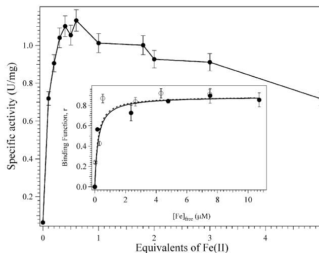
FIGURE 1: Plot of specific activity (U/mg) of H178A EcMetAP-I vs equivalents of Fe(II). Activity assays were performed with 8 mM MGMM in 25 mM HEPES, pH 7.5, 150 mM KCl. Inset: Plot of binding function, r , vs free Fe(II) concentration, [\text{Fe}]_{\text{free}} , for WT EcMetAP-I (○) and H178A EcMetAP-I (●). The solid line represents a fit of Fe(II) activity titration data for H178A EcMetAP-I to eq 1. This fit provided a value of p = 1 and a K_{\text{d}} value of 0.30 \pm 0.15 \mu\text{M} (Figure 1). These data are identical, within error, to those obtained for Fe(II) binding to WT EcMetAP-I (dashed line, K_{\text{d}} = 0.20 \pm 0.15 \mu\text{M} ).
