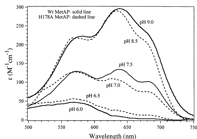
FIGURE 6: Electronic absorption spectra of Co(II)-loaded WT (solid line) and H178A (dashed line) EcMetAP-I . Visible spectra were recorded at various pH for 1 mM WT and H178A EcMetAP with one equivalence of Co(II).
